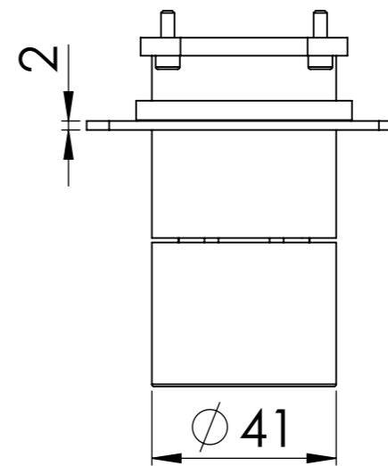
CONNESSIONE CARTUCCIA R52APWBAA R52APWBAA CARTRIDGE CONNECTION
