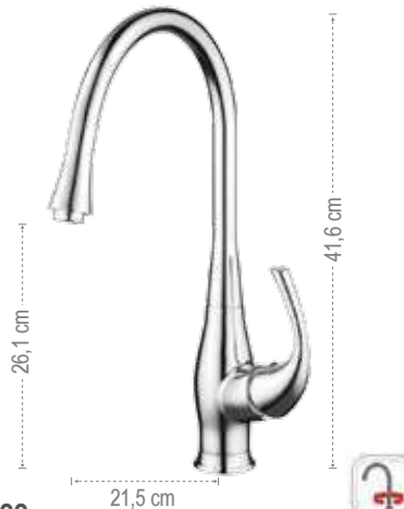
U422 Monocomando lavello con bocca alta girevole. Single lever kitchen mixer with high swivel spout.
