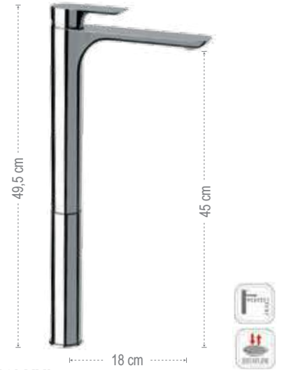
I10LXXL Miscelatore monocomando lavabo alto XXL, con scarico click-clack con troppo-pieno. XXL high single-lever basin mixer, with click-clack waste and overflow.
