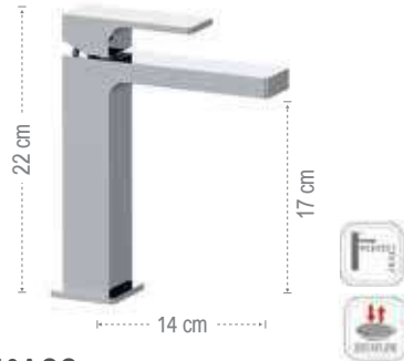
AU10ACC Miscelatore monocomando per lavabo, modello "A" altezza media, scarico click-clack con troppo-pieno incluso. Single-lever basin mixer, model "A" medium height, click-clack waste with overflow included.
