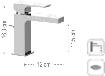
AU10 Monocomando lavabo, con scarico. Single-lever basin mixer, with pop-up waste.
