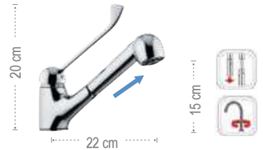
K47LL Miscelatore monocomando per lavello con leva lunga e doccia estraibile a getto variabile. Single-lever one-hole sink mixer with long lever and with pull-out spray jet shower with 2 functions.
