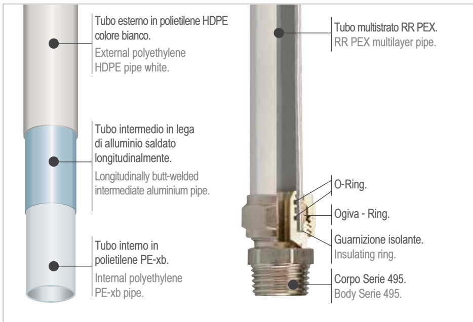
Tubo multistrato RR PEX. Multilayer pipe RR PEX.
