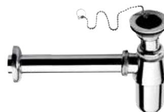
Sifone a bottiglia in zama con pileta, per lavabo, 1" 1/4. Bottle trap in zamac with waste, for wash-basin, 1" 1/4.
