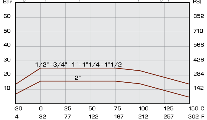
Diagramma pressione/temperatura - Pressure/temperature graph
