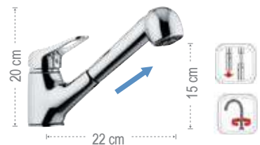
K47M Miscelatore monocomando monoacqua per lavello, con doccia estraibile a getto variabile. Single-lever single water one-hole sink mixer, with pull-out spray jet shower two functions.
