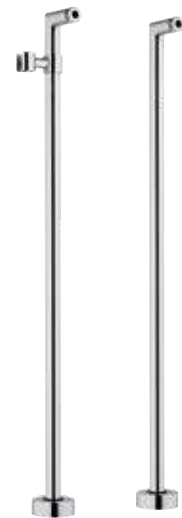
88N02 Coppia colonne vasca in ottone, serie Minimal, con supporto doccia, 3/4M x 3/4M. Couple brass vertical connections for bath mixer, serie Minimal, with handshower holder 3/4M x 3/4M.
